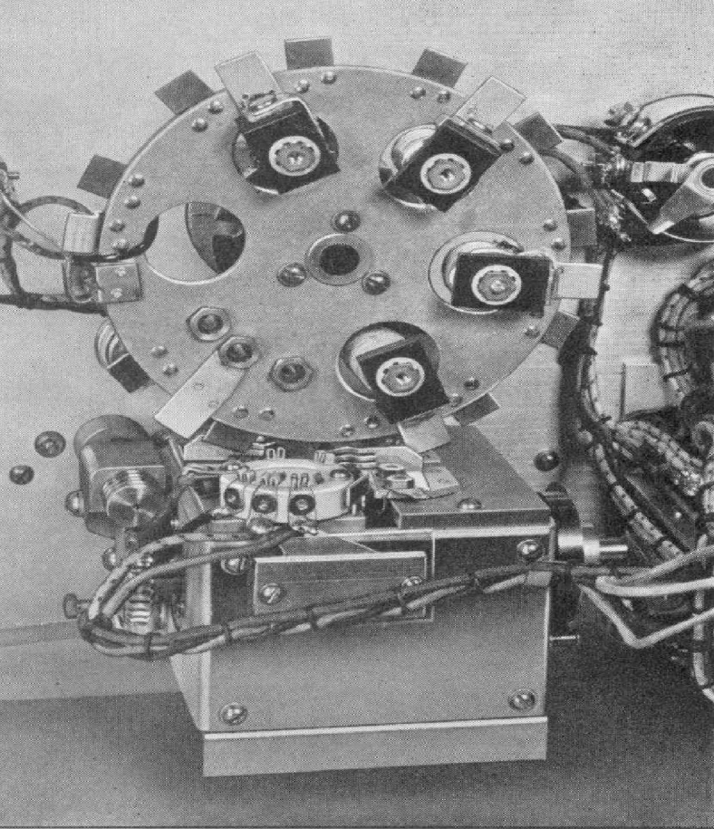
FIGURE 4. Rear view of the coil switching mechanism. A positive wiping contact between silver-plated surfaces is obtained. Leads are made short and direct in order to keep residual inductance and capacitance low.
