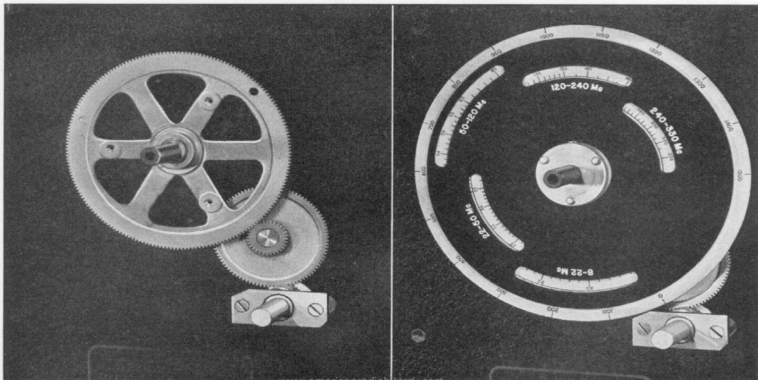
FIGURE 3. Two views of the frequency-control drive mechanism partially disassembled. In the left-hand view are shown the gears through which the direct-reading frequency dial is driven from the worm shaft of the condenser. The dial attaches directly to the large gear. At the right, the dial and mask are shown assembled. The bakelite shaft concentric with the large gear drives both the coil switch and the mask for the frequency scales.
