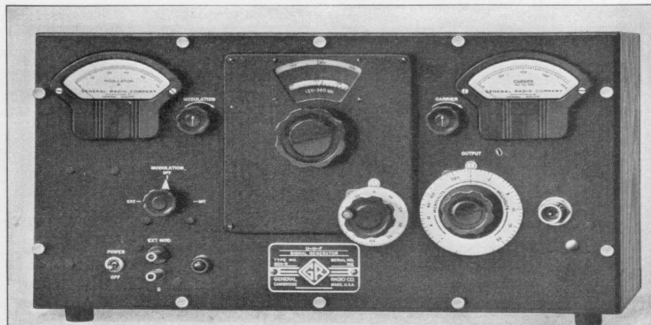
FIGURE 1. Panel view of the TYPE 804-B U-H-F Signal Generator. The knob in the center controls the band-change switch, and the dial below it, the tuning condenser. The output control is at the lower right.
