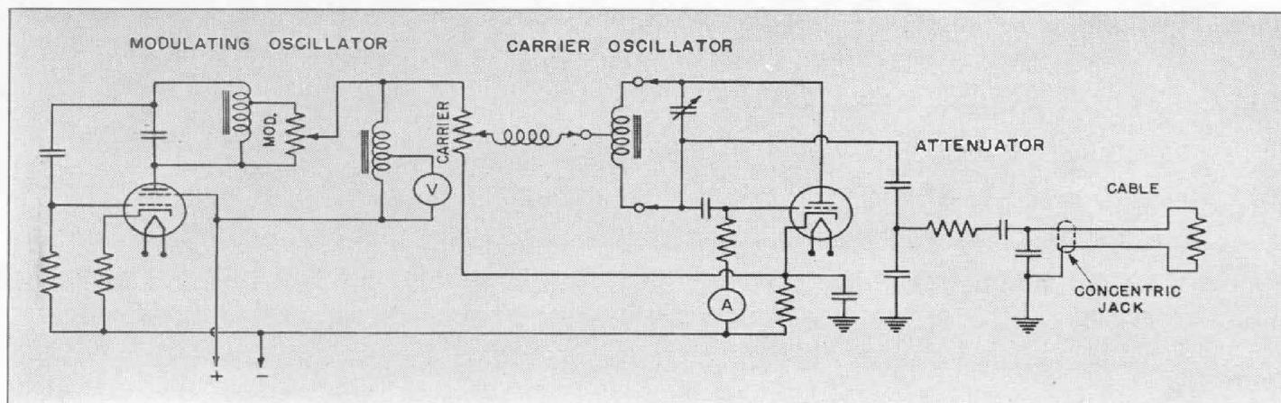
FIGURE 2. Schematic circuit diagram of TYPE 804-B U-H-F Signal Generator. The a-c power supply is not shown.
